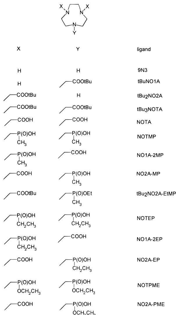
Figure 1. Ligands discussed in this study.
