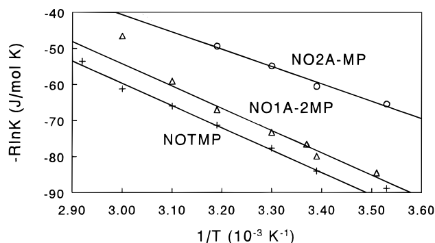
Figure 5. – R ln K eq ( K eq is defined for the equilibrium \text{MgL} + \text{H}^+ \rightleftharpoons \text{Mg}^{\text{II}} + \text{HL} ) versus 1/ T for NOTMP ([L] tot = 2.00 mM, [Mg] tot = 2.00 mM), and NO1A-2MP and NO2A-MP ([L] tot = 2.00 mM, [Mg] tot = 1.62 mM), as determined by variable temperature 31 P NMR (202 MHz) at pH 7.4. The slopes represent Δ H values for this equilibrium.
