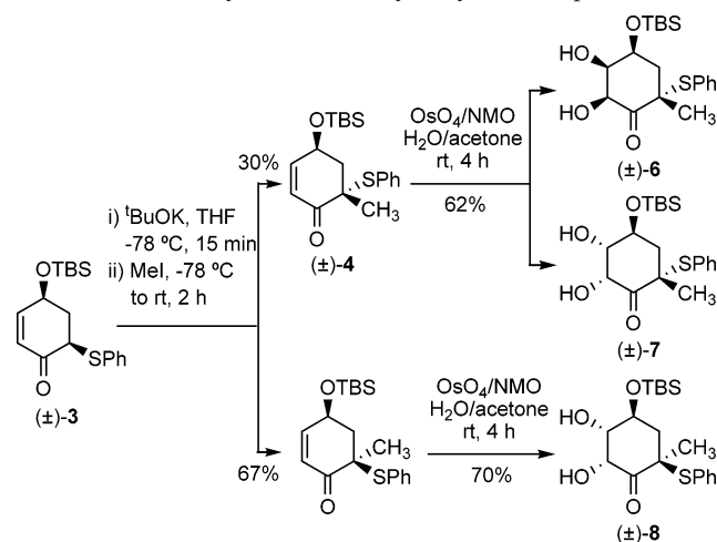
Scheme 3. Partial Synthetic Sequence to Gabosines O and N: The Alkylation and Dihydroxylation Steps
