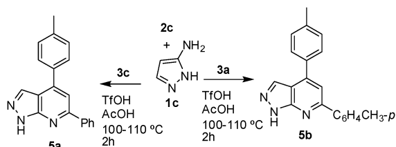
Scheme 1 The synthesis of pyrazolo[3,4- b ]pyridine derivatives.
