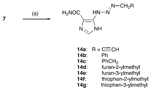
Scheme 3. Synthesis of 1-substituted-3-(4-carbamoylimidazol-5-yl)triazenes ( 14 ). Reagents and Conditions: a) RCH 2 NH 2 , EtOAc, 25 °C.
