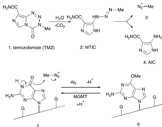
Scheme 1. Structures of temozolomide (1) and MTIC (2), the formation of \text{O}^6 -methylguanine residues (6) in DNA at runs of guanines (G) and repair of methylated DNA by \text{O}^6 -methyl-DNA methyltransferase (MGMT).
