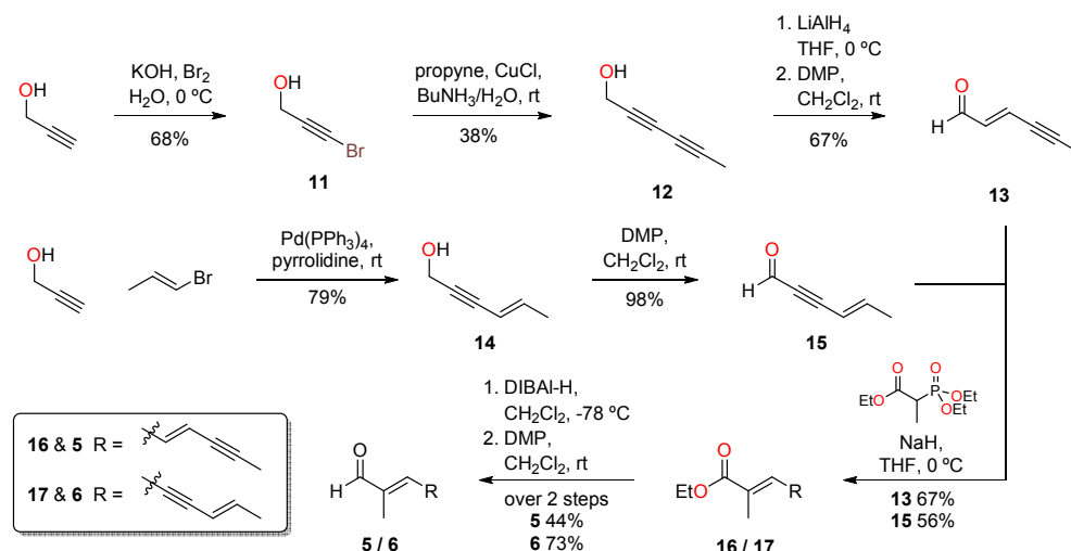
Scheme 3. Final steps of the synthesis of 2 and 3.
