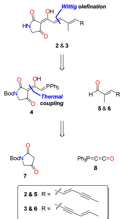
Figure 2. Retrosynthetic pathway for putative co-metabolites 2 and 3 .
