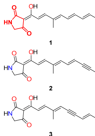
Figure 1. Ravenic acid ( 1 ), with the tetramic acid core highlighted in red, and possible structures for unknown co-metabolite ( 2 & 3 ).
