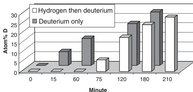
Figure 4. Comparison of 7,8-benzoquinoline deuteration with and without 1 h pre-incubation with hydrogen gas
