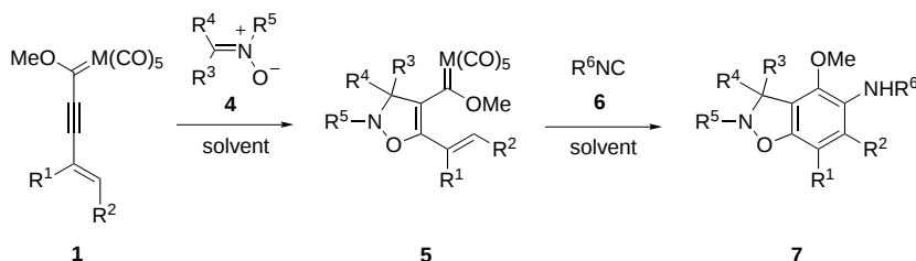
Scheme 3. Preparation of 1,3,5-metallahexatrienes 5 and their cyclization to afford 2,3-dihydro-1,2-benzisoxazoles 7 .
