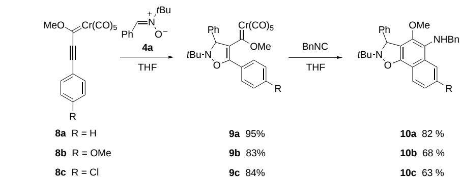
Scheme 4. Preparation of 1,3,5-metallahexatrienes 9 and their cyclization to afford naphthoisoxazole derivatives 10 .
