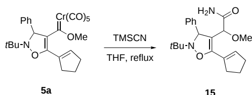
Scheme 7. Preparation of amide 15 by reaction of metallahexatriene 5a and trimethylsilyl cyanide.
