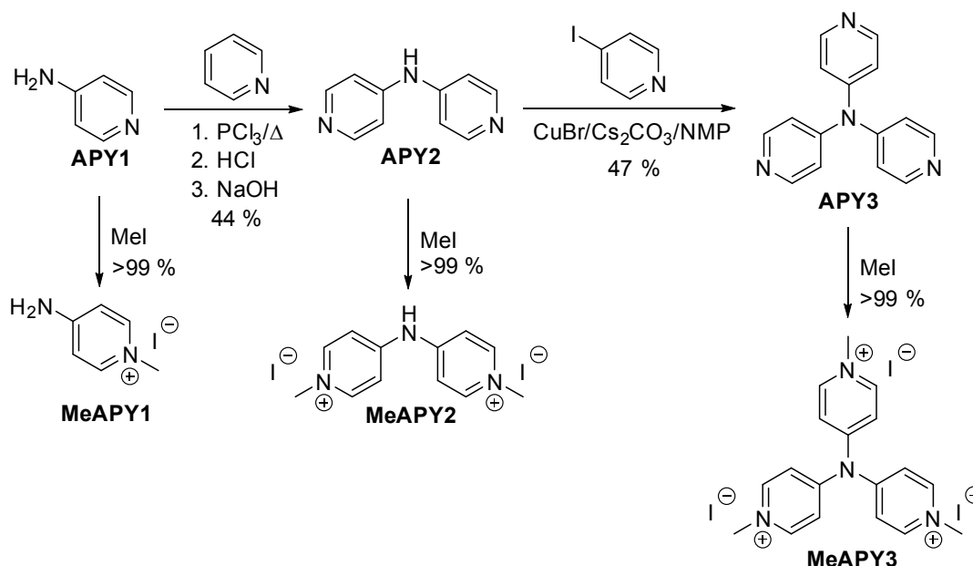
Scheme 1 Synthesis of aminopyridines (APY) and aminopyridiniums (MeAPY)
