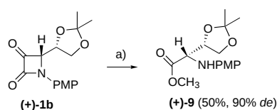
Scheme 7. One-step preparation of \alpha -amino ester 9 from azetidine-2,3-dione 1a and sodium methoxide/methanol. a) MeONa, MeOH, RT.
