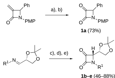
Scheme 2. Preparation of azetidine-2,3-diones 1a–d . a) \text{OsO}_4 , \text{Me}_3\text{NO} , acetone/water, RT. b) \text{NaIO}_4 , \text{NaHCO}_3 , dichloromethane, RT. c) \text{Et}_3\text{N} , \text{AcOCH}_2\text{COCl} , dichloromethane, RT. d) \text{NaOCH}_3 , \text{CH}_3\text{OH} , 0^\circ\text{C} . e) i) (\text{CO})_2\text{Cl}_2 , DMSO, dichloromethane, -78^\circ\text{C} , 2 h, ii) \text{Et}_3\text{N} .
