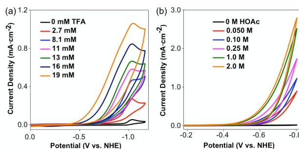
Figure 1. CVs of (a) 1.0 mM of 6a in 0.10 M n -Bu 4 NPF 6 in DMF with different concentrations of TFA; (b) 1.0 mM 6a in 0.10 M Na 2 SO 4 with different HOAc concentrations at scan rates of 100 mV s -1 with a glassy carbon working electrode ( 3 mm diameter).
