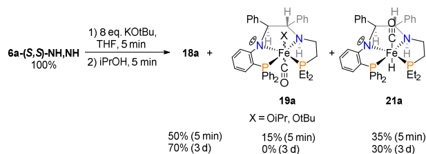
Scheme 8 Products of the activation of 6a .
