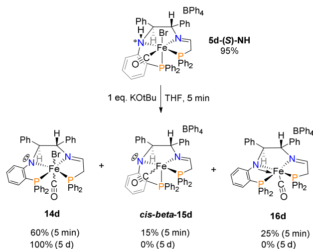
Scheme 4 Reaction of 5d with one equivalent of KOTBu.
