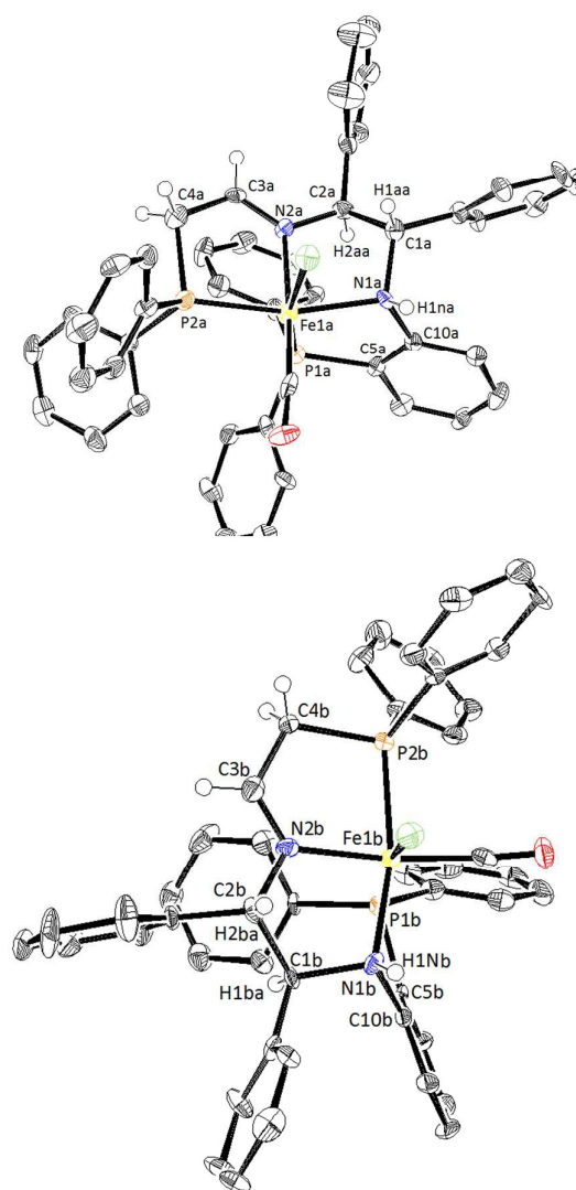
Fig. 4 ORTEP plot of 5d containing the pair of diastereomers, with (R)-NH on the top and (S)-NH on the bottom. The molecules have been rotated to display the difference in the gauche and anti -conformation of the (R)-NH and (S)-NH, respectively with respect to the CH of the adjacent CHPh group. Thermal ellipsoids are drawn at 50% probability level. Aromatic ring protons and the BPh 4 counteranions were omitted for clarity. Selected interatomic distances (Å) and angles (deg): For (R)-NH: Fe1a-N2a 2.077(8), Fe1a-N2a 1.976(8), F1a-P1a 2.247(3), Fe1a-P2a 2.233(3), N1a-C10a 1.440(12), P1a-C5a 1.819(10), N2a-C3a 1.275(11), C3a-C4a 1.485(14), N1a-C1a 1.521(11), N2a-C2a 1.485(10); P1a-Fe1a-P2a 103.80(13). For (S)-NH: Fe1b-N1b 2.047(9), Fe1b-N2b 1.982(8), Fe1b-P1b 2.260(3), Fe1b-P2b 2.248(3), N1b-C10b 1.472(12), P1b-C5b 1.823(10), N2b-C3b 1.263(11), C3b-C4b 1.476(14), N1b-C1b 1.545(10), N2b-C2b 1.497(10); P1b-Fe1b-P2b 102.00(13).
