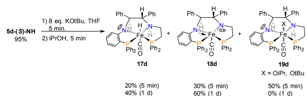
Scheme 5 Products of the activation of 5d .
