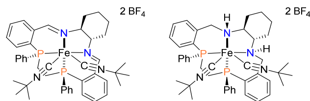
Fig. 3 Selected cis-β iron (II) PNNP complexes developed in the Mezzetti group.
