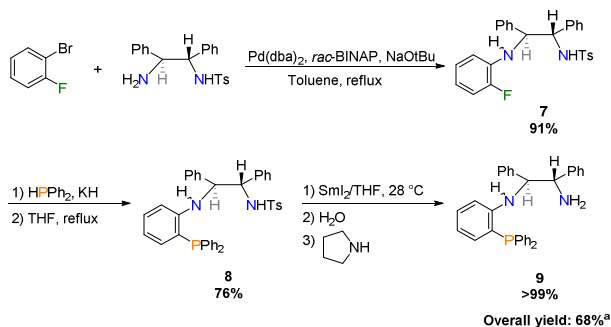
Scheme 1 Synthesis of BenzoPPh 2 DPEN ( S,S ) isomer 9 . a Percent overall yield was calculated based on molar amount of monotosylated-( S,S )-DPEN.
