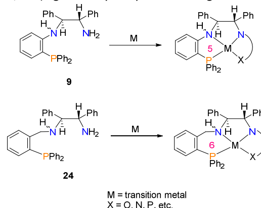
Scheme 10 Employing 9 as a substitute for the commonly used ligand 24 to shorten the metallocycle ring size by one.
