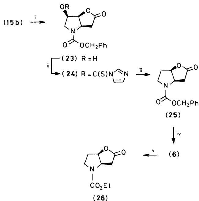
Scheme 3. Reagents and conditions: i, 80% \text{CF}_3\text{CO}_2\text{H} , room temp., 18 h; ii, 1,1'-thiocarbonyldi-imidazole, \text{C}_5\text{H}_5\text{N} , THF, reflux; iii, \text{Bu}_3\text{SnH} (2.2 mol equiv.), \text{C}_6\text{H}_6 , reflux; iv, 10% Pd/C, \text{H}_2 , EtOH, HCl; v, \text{ClCO}_2\text{Et} , \text{Et}_3\text{N} , \text{CH}_2\text{Cl}_2 , 0^\circ\text{C} to room temp.
