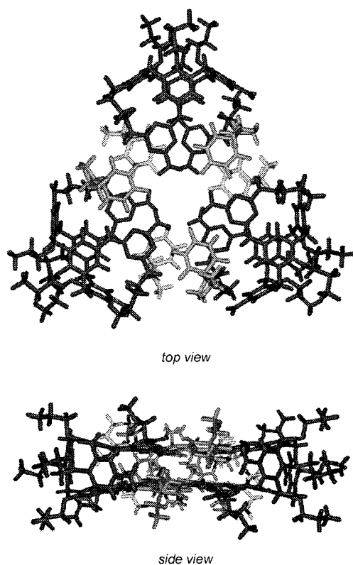
Figure 3. X-Ray crystal structure of 1b_3 \cdot (DEB)_6 . [24]
