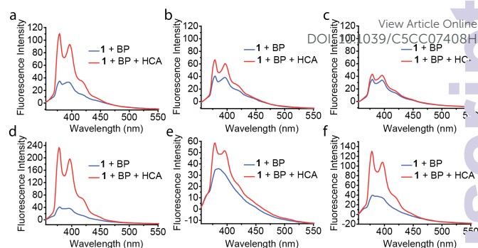
Figure 4. Fluorescence spectra of probe 1 (1 \mu\text{M} ) and benzophenone (5 mM) treated without or with 1 \mu\text{M} HCA in different surfactant solutions: (a) 1 mM Brij 35; (b) 5 mM Brij 35; (c) 20 mM Brij 35; (d) 4 mM Triton X-100; (e) 1 mM Tween 20; (f) 1 mg/mL PE6-12-dodecyl random copolymer. All experiments were carried out in Tris buffer solution (25 mM, pH 7.4). All spectra were taken after 3-hour protein incubation at room temperature.
