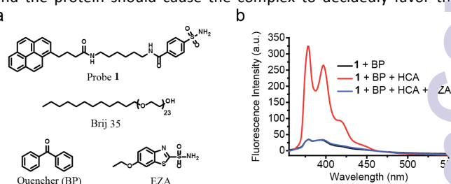
Figure 2. (a) Chemical structures of probe 1, quencher and micelle. (b) Fluorescence spectra of probe 1 (1 μM) and benzophenone (5 mM) in Brij 35 (1 mM) Tris buffer solution (25 mM, pH 7.4) treated without or with HCA (5 μM) or with HCA (5 μM) and EZA (100 μM). All spectra were taken after 3-hour HCA incubation at room temperature.
