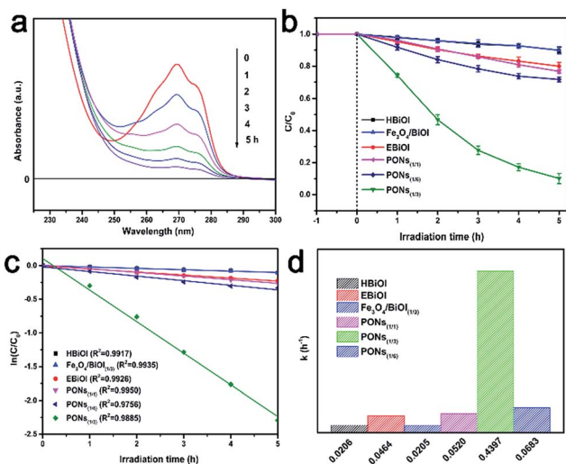
Fig. 9 (a) The time-dependent absorption spectra of phenol in the presence of PONS (1/3) under visible-light irradiation (λ > 420 nm). (b) Degradation ratios, (c) first-order kinetics data and (d) rate constants for the photocatalytic removal of phenol by various photocatalysts under visible-light irradiation.
