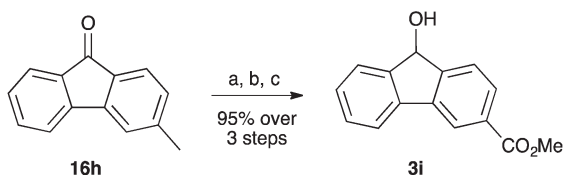
Scheme 6 The conversion of 3-methylfluorenone 16h to the methyl ester 3i . (a) KMnO 4 , Py/H 2 O, Δ; (b) cat. H 2 SO 4 , MeOH, Δ; (c) NaBH 4 , MeOH, 0 °C.
