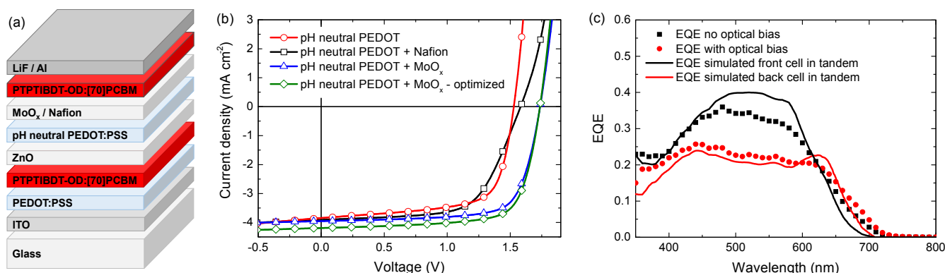
Fig. 4 (a) Layout of the PTPTIBDT-OD:[70]PCBM homo-tandem polymer solar cell with Nafion or \text{MoO}_3 layers in the intermediate contact. (b) Comparison of the J-V characteristics of PTPTIBDT-OD:[70]PCBM homo-tandem solar cells with and without Nafion or \text{MoO}_3 layers in the intermediate contact. (c) EQE measurement of a PTPTIBDT-OD:[70]PCBM homo-tandem cell with and without optical bias (markers) in comparison with simulated EQEs of the subcells inside the tandem cell (solid lines).
