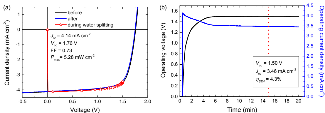
Fig. 5 (a) J - V curves of the PPTIBDT-OD:[70]PCBM homo-tandem cell before, during, and after the 20 min. light-driven electrochemical water splitting experiment. (b) Simultaneous measurement of operating voltage and current density of the device during light-driven electrochemical water splitting using \text{RuO}_2 catalysts in 1.0 M KOH. The light source is not chopped and the electrolyte is not stirred during measurements.
