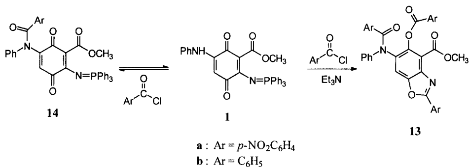
Scheme 5
