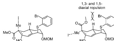
FIGURE 3. Stereoelectronic controlled elaboration of the C-7 quaternary center.
