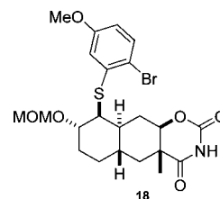
FIGURE 4. The relative stereochemistry of the oxazine-2,4-dione 18 .
