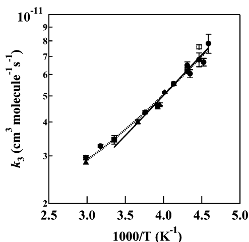
Figure 5. Plot of the k_3 value (on a logarithmic scale) from this work versus 1/T . Dotted line is a weighted least-squares fit to the equation k_3(T) = AT^2 \exp[-E_a/(RT)] and yields k_3(T) = (8.79 \pm 0.67) \times 10^{-19} T^2 [\exp((1130 \pm 20)/T)] cm 3 molecule -1 s -1 . Solid line is a fit to the data at T \leq 298 K (shown in the figure over that range) to an Arrhenius expression, which yields k_3(T) = (3.2 \pm 0.3) \times 10^{-13} \exp[(690 \pm 40)/T] cm 3 molecule -1 s -1 . All the quoted errors are 2 \sigma precision obtained via least-squares analyses.
