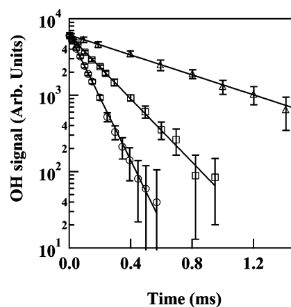
Figure 2. Typical OH temporal profiles recorded at 242 K in the presence of various concentrations of PNA: (○) 1.4 \times 10^{15} \text{ molecule cm}^{-3} , (□) 6.9 \times 10^{14} \text{ molecule cm}^{-3} , and (△) 2.1 \times 10^{14} \text{ molecule cm}^{-3} . Solid lines are weighted linear least-squares fits of the data to eq 1.
