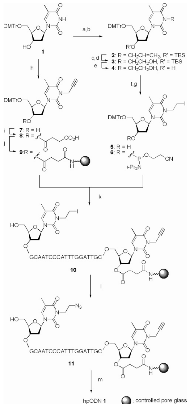
SCHEME 1. Preparation of hpODN 1 Containing N -3-(Propargyl)thymidine and N -3-(Azidoethyl)thymidine Derivatives a
