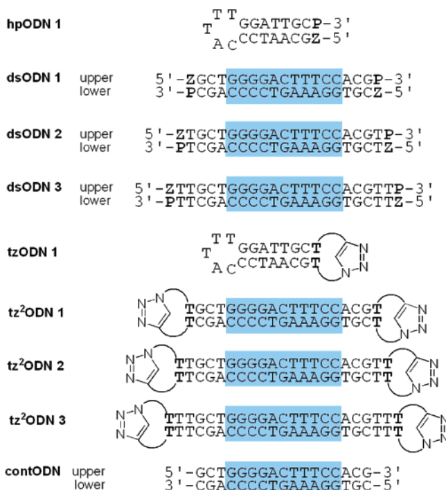
FIGURE 2. Sequences of the ODNs used in this study. P = N -3-(propargyl)thymidine residue; Z = N -3-(azidoethyl)thymidine residue; T = N -3-substituted thymidine residue. NF- \kappa B recognition regions are marked with a gray box.
