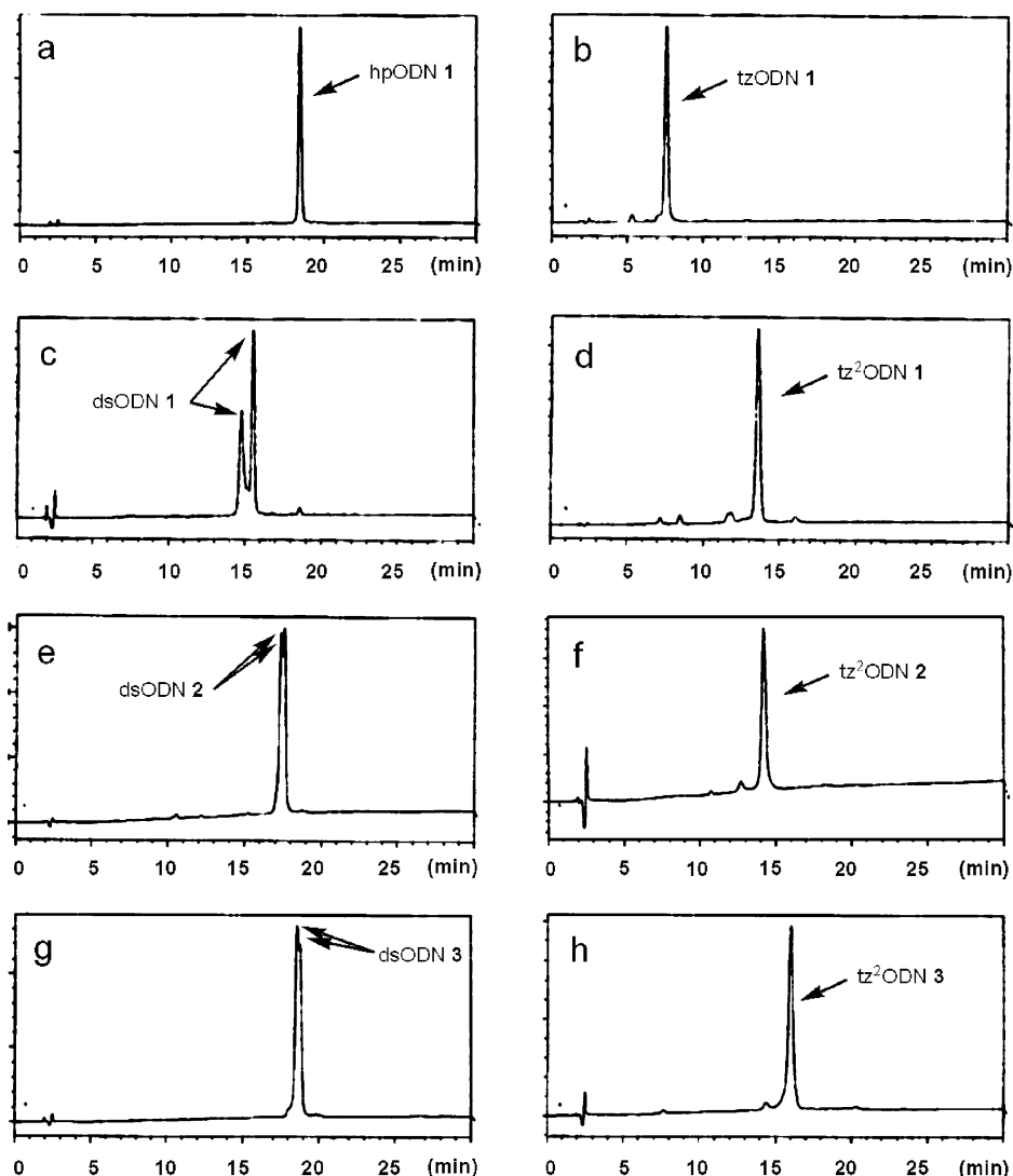
FIGURE 3. Denaturing reverse-phase HPLC chromatograms (UV absorbance vs time) of the cross-linking reaction of hpODN 1 and dsODNs 1, 2, and 3: (a) hpODN 1 in the absence of Cu[I] catalysis; (b) after the CuAAC of hpODN 1; (c) dsODN 1 in the absence of Cu[I] catalysis; (d) after the CuAAC of dsODN 1; (e) dsODN 2 in the absence of Cu[I] catalysis; (f) after the CuAAC of dsODN 2; (g) dsODN 3 in the absence of Cu[I] catalysis; (h) after the CuAAC of dsODN 3. All the reactions were performed with 50 \mu M ODN in 100 mM NOPS–NaOH (pH 7, 1 M NaCl– t BuOH) in the presence of 500 mM CuSO 4 –TBTA complex and 5 mM sodium ascorbate for 6 h to afford tzODN 1 and tz 2 ODN 1, 2, and 3 (indicated as arrows), respectively.
