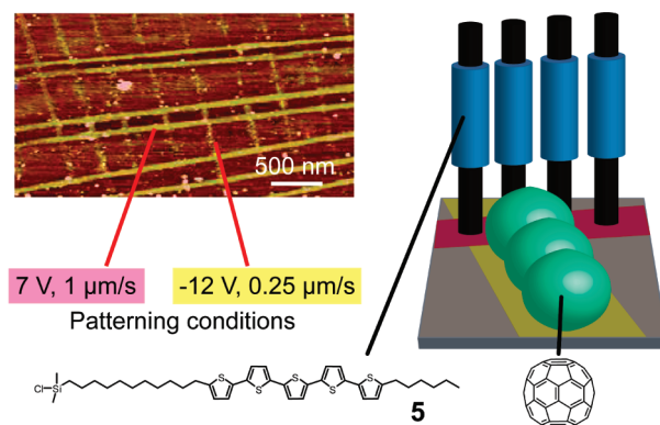
Figure 3. Multiplexed directed assembly onto bifunctionally patterned 3 . (left) AFM height image (Z axis = 10 nm). (right) Graphical representation of the assembled surface, with C 60 deposited on the reductive patterns (−12 V, 0.25 μm/s) and 5 deposited on the oxidative patterns (7 V, 1 μm/s). All of the patterns were drawn at 70% relative humidity.
