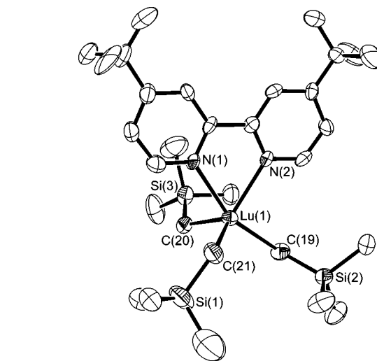
Figure 1. Molecular structure of 4 (left) with thermal ellipsoids projected at the 50% probability level. Selected bond distances (Å) and angles (deg): \text{Lu}(1)-\text{N}(1) = 2.437(7) , \text{Lu}(1)-\text{N}(2) = 2.427(7) , \text{Lu}(1)-\text{C}(19) = 2.369(8) , \text{Lu}(1)-\text{C}(20) = 2.358(9) , \text{Lu}(1)-\text{C}(21) = 2.318(9) ; \text{N}(1)-\text{Lu}(1)-\text{N}(2) = 65.7(2) , \text{Lu}(1)-\text{C}(19)-\text{Si}(2) = 139.5(5) , \text{Lu}(1)-\text{C}(20)-\text{Si}(3) = 120.8(4) , \text{Lu}(1)-\text{C}(21)-\text{Si}(1) = 126.1(5) .
