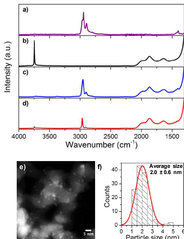
Figure 1. FT-IR spectra of a) [\text{Cu}_4(\text{HMDS})_4] , b) \text{SiO}_2\text{-700} , c) [\text{CuHMDS}]/\text{SiO}_2\text{-TMS} , d) \text{Cu}/\text{SiO}_2\text{-TMS} ( 1 ) and e) HR-TEM image and f) particle size distribution of 1 .
