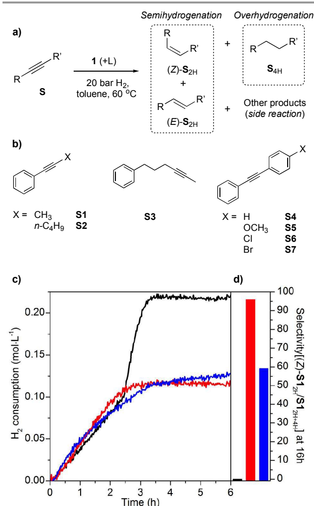
Figure 2. Hydrogenation of alkynes with catalyst 1 . a) General reaction scheme, b) substrate scope, c) H_2 consumption profiles for hydrogenation of 1-phenyl-1-propyne ( S1 , 400 \mu mol) at 20 bar, 60 °C in toluene over unmodified 1 (black, 1.8 mol% Cu total ) or in the presence of IMes (red) or PCy 3 (blue) using a molar ratio ligand/ S1 = 1:50, and d) selectivity to (Z)- S1 2H among hydrogenation products S1 2H and S1 4H (selectivity[(Z)- S1 2H / S1 2H+4H ]) at final time (16 h).
