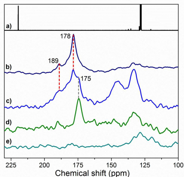
Figure 3. (a) 13 C NMR solution-state spectrum of free IMes* (C 6 D 6 , 75 MHz); (b) 13 C NMR solid-state HPDEC spectrum of 2* (30000 scans); 13 C NMR solid-state CP-MAS spectra of (c) 2* (90000 scans), (d) IMes*/SiO 2-TMS (27513 scans) and (e)
