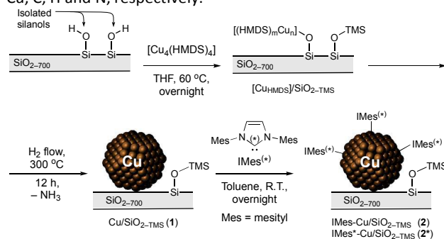
Scheme 1. Synthetic route to 1 and 2 .
