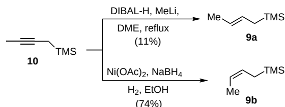
Scheme 3. Synthesis of \gamma -substituted allylsilanes 9a and 9b .
