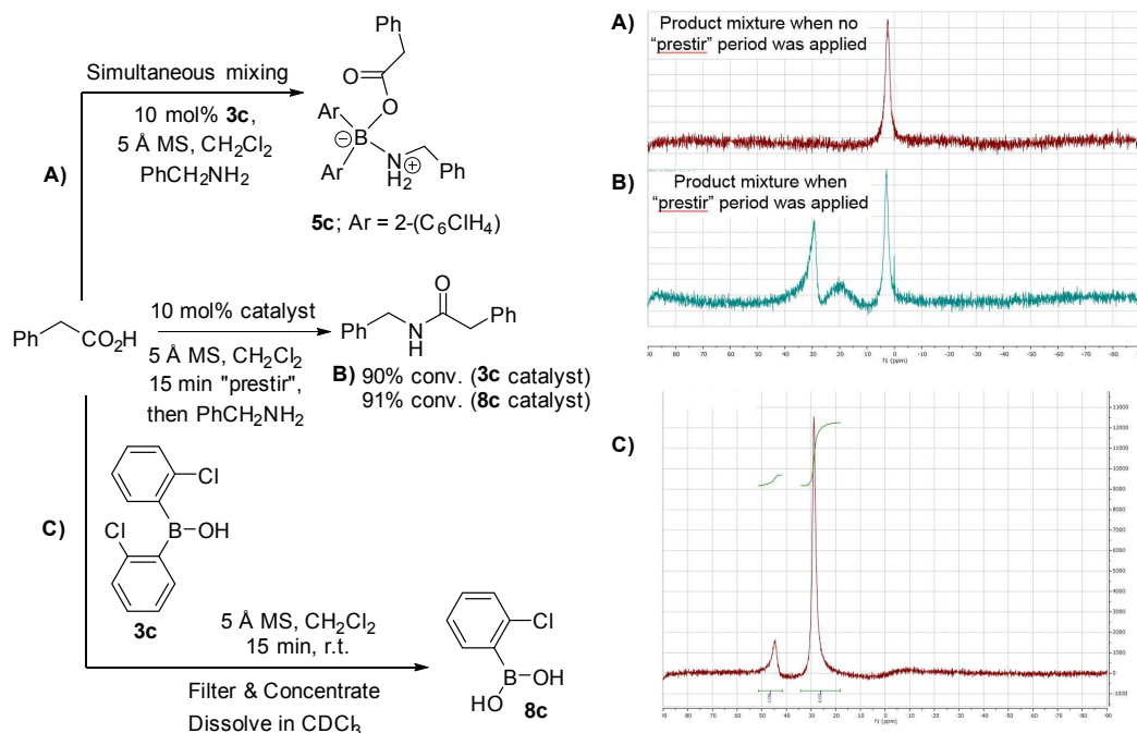
Scheme 6. Examining bis-2-chlorophenylborinic acid 3c as a catalyst for direct amide formation and ^{11}\text{B} NMR spectra of product mixtures obtained in 3 examined cases.
