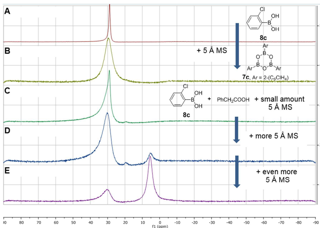
Figure 7. ^{11}\text{B} NMR spectra showing interactions between 2-chlorophenylboronic acid 8c , phenylacetic acid and 5 Å MS. A: 2-chlorophenylboronic acid; B: addition of 5 Å MS to ( A ), leading to boroxine formation; C: addition of a tiny amount of 5 Å MS to a mixture of boronic and carboxylic acid; D: addition of more 5 Å MS; E: addition of even more 5 Å MS.
