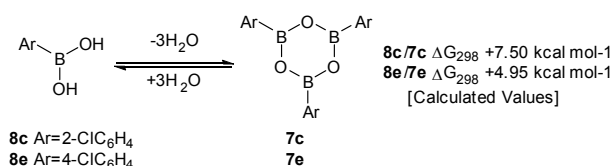
Scheme 9. Calculated ΔG 298 values for the formation of boroxines from o -chlorophenylboronic 8c acid and p -chlorophenylboronic acid 8e .
