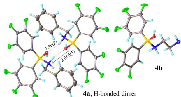
Figure 1. X-ray structures of Lewis adducts 4a (H-bonded dimer) and 4b .
