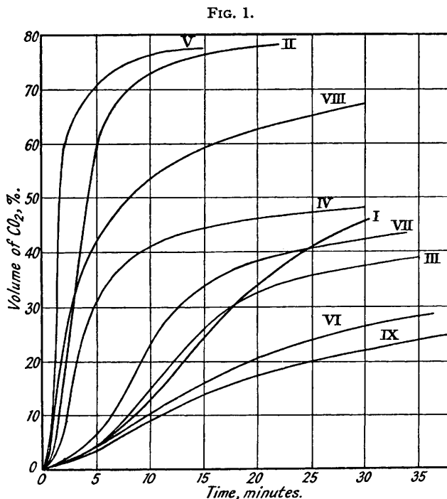
Formate: I, Triphenylmethyl. II, o -Methoxytriphenylmethyl. III, m -Methoxytriphenylmethyl. IV, p -Methoxytriphenylmethyl. V, 2:2'-Dimethoxytriphenylmethyl. VI, 3:4-Dimethoxytriphenylmethyl. VII, 3:4:5-Trimethoxytriphenylmethyl. VIII, 2-Methoxy-4'-methyltriphenylmethyl. IX, Diphenyl- p -diphenylmethyl.
