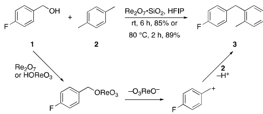
Scheme 1. \text{Re}_2\text{O}_7 -mediated dehydrative Friedel-Crafts alkylation.
