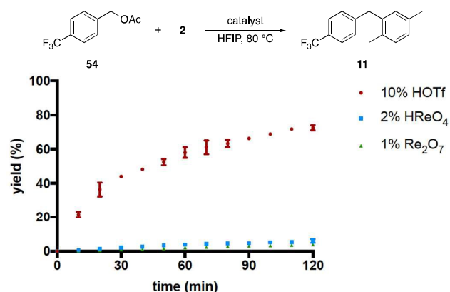
Figure 3. Acetate ionization by different catalysts.
