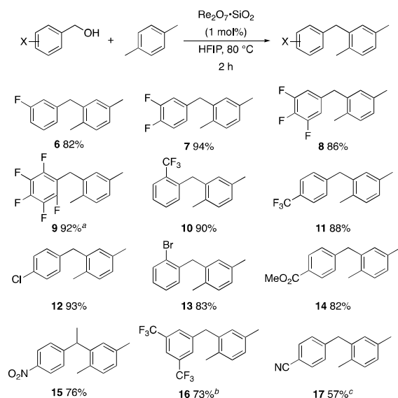
Figure 1. Representative scope of the dehydrative diarylmethane synthesis. a Reaction was conducted at 100 °C for 24 h. The product was isolated in 95% yield when the reaction was conducted at 80 °C for 5 h with crystalline \text{Re}_2\text{O}_7 . b Reaction was conducted with crystalline \text{Re}_2\text{O}_7 for 23 h. c Reaction was conducted with crystalline \text{Re}_2\text{O}_7 for 48 h.
