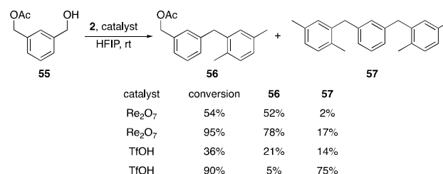
Scheme 7. Reactions with a difunctionalized substrate.
