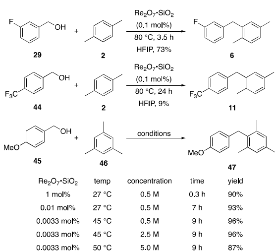
Scheme 3. Reactions at lower catalyst loading.
