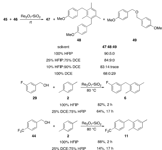
Scheme 4. Solvent effects.
