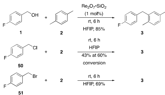
Scheme 5. Leaving group comparison.
