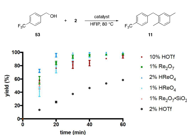
Figure 2. Reaction kinetics as a function of catalyst.
