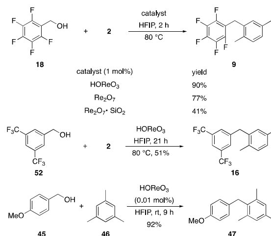
Scheme 6. Catalyst comparison.
