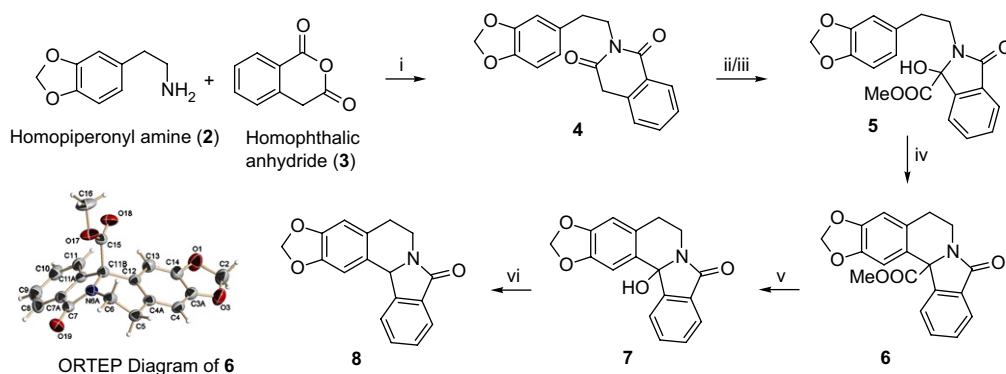
Scheme 1. Synthesis of isoidoloisoquinoline. Reagents, conditions, and yields: (i) o -dichlorobenzene, reflux, 3 h (92%); (ii) NaBH 4 , MeOH, rt, 20 h (70%); (iii) MeOH, NEt 3 , rt, 12 h (76%); (iv) 6 M H 2 SO 4 +AcOH (1:2), rt, 2 h (84%); (v) NaCl, H 2 O, DMSO, 175 °C, 30 min (79%); (vi) NaBH 4 , TFA, rt, 5 h (85%).
