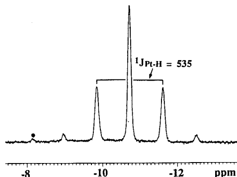
Figure 4. High-field region of the 1 H NMR spectrum of [ trans,cis -(C 6 F 5 ) 2 (PPh 3 )Pt(μ-H)(μ(P)-η 2 -PPh 3 )Pt(C 6 F 5 ) 2 ] ( 2a ) in CD 3 COCD 3 at 20 °C. The signal denoted with an asterisk is due to a small amount of 2c ; J is in hertz.
