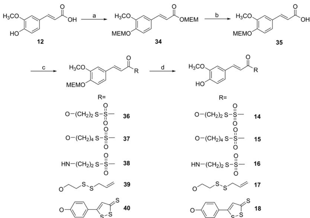
Scheme 2. Reagents and conditions: (a) MEM-Cl, DIPEA, anh. \text{CH}_2\text{Cl}_2 , 5 h, 0^\circ\text{C} to r.t.; (b) \text{LiOH}\cdot\text{H}_2\text{O} , THF/ \text{H}_2\text{O} (2:1), 24 h, r.t.; (c) RH (1–5), DCC (EDAC for 38), DMAP, anh. \text{CH}_2\text{Cl}_2 ( \text{CHCl}_3 for 38), 3–20 h, r.t.; (d) TFA, anh. \text{CH}_2\text{Cl}_2 , 4–7 h, r.t.
