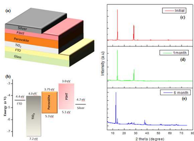
Figure 3. (a) Schematic device structure; (b) Energy level diagram of the different materials used in the device; (c) X-ray Diffraction (XRD) analysis plot of \text{CH}_3\text{NH}_3\text{PbI}_{3-x}\text{Cl}_x films at initial stage, (d) that after one month storage and (e) after 6 months storage.
