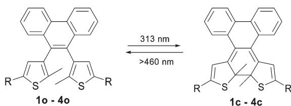
Scheme 3 Reversible switching upon irradiation.
