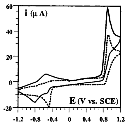
Figure 2. Cyclic voltammograms of \text{CH}_3\text{AHt-Bu} (2 mM) in the absence (dotted line) and presence (full line) of a strong base (0.17 M 2,4,6-trimethylpyridine) in acetonitrile + 0.1 M \text{Bu}_4\text{NBF}_4 at 20°C. Successive potential scans from 0 to 1.2 V, from 1.2 to -1.2 V and from -1.2 to 0 V at \nu = 0.2 \text{ V s}^{-1}
