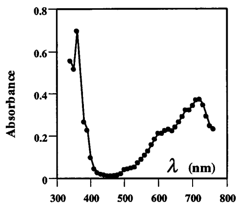
Figure 1. Absorption spectrum of \text{CH}_3\text{AHt-Bu}^{+\bullet} in acetonitrile recorded 1 ms after the pulse. \text{CH}_3\text{AHt-Bu} (0.16 mM) + 0.1% \text{CCl}_4 ; 120 mJ laser pulse at 308 nm
