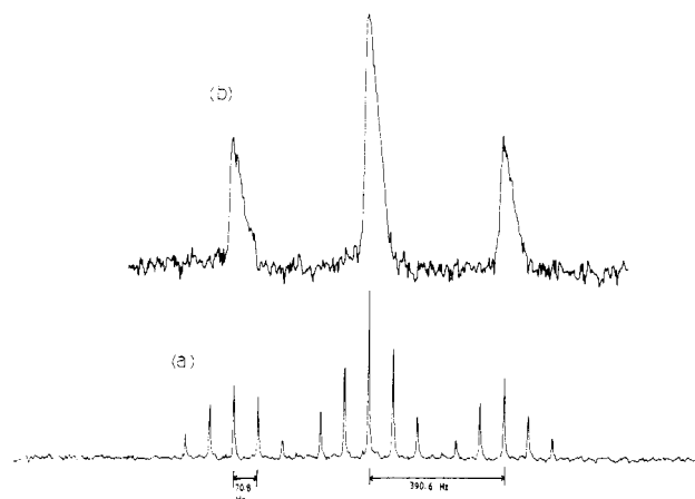
Figure 1. ^{195}\text{Pt} NMR spectra of 0.57 M cis -[Pt( ^{15}\text{NH}_3 ) 2 (H 2 O) 2 ](ClO 4 ) 2 in H 2 O: (a) without ^1\text{H} decoupling; (b) with ^1\text{H} decoupling. Conditions were as defined in the Experimental Section, except that there were only 200 scans and 16K data points at 20 KHz width.
