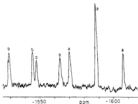
Figure 2. ^{195}\text{Pt} NMR spectrum of a solution containing cis -Pt( ^{15}\text{NH}_3 ) _2(\text{H}_2\text{O})_2^{2+} (I) (peaks labeled "a") and (\text{Pt}(^{15}\text{NH}_3)_2(\text{H}_2\text{O}))_2(\mu\text{-OH})^{3+} (II) (peaks labeled "b") at pH 3.
