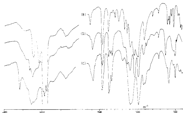
Figure 5. IR spectra of Nujol mulls of (a) \text{Pd(en)(PO}_4\text{H)} , (b) white \text{Pt(NH}_3)_2(\text{PO}_4\text{H})\cdot 0.5\text{H}_2\text{O} , (c) blue \text{Pt(NH}_3)_2(\text{PO}_4\text{H})\cdot 0.5\text{H}_2\text{O} ( \times = Nujol peaks).
