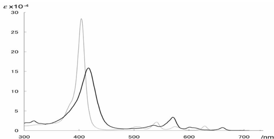
Figure 4. UV-vis spectra of thiabenzoporphyrin 20 (bold line) and benzoporphyrin 21 (solid line)
