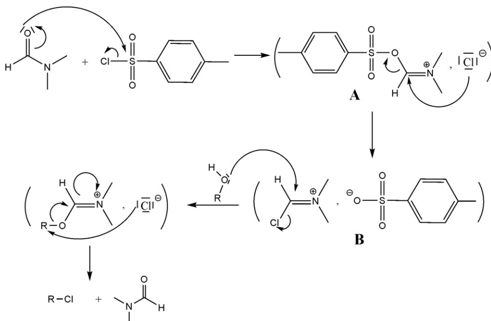
Scheme 3. Proposed mechanism of selective chlorination.
