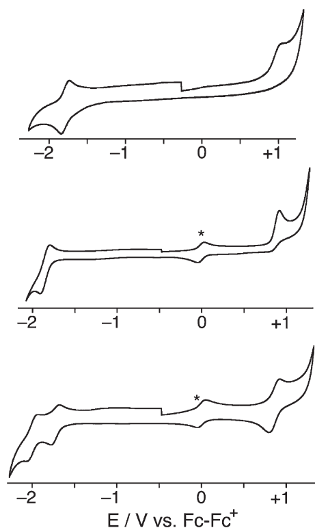
Fig. 13 Cyclic voltammograms of (a) Pt-PBE-Ph ; (b) Re-PBPh ; (c) Ru-PBN in \text{CH}_2\text{Cl}_2 at a scan rate of 500 \text{ mV s}^{-1} with a Pt disk working electrode. * denotes the redox couple of ferrocene which was added as an internal reference.
