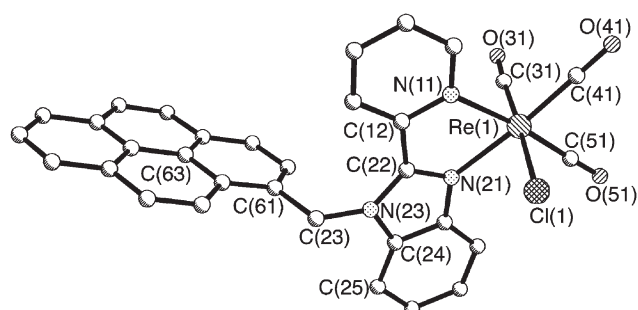
Fig. 3 Molecular structure of Re-PBPyr .
