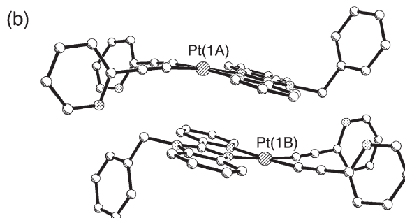
Fig. 6 Molecular structure of Pt-PBPh-Py .
