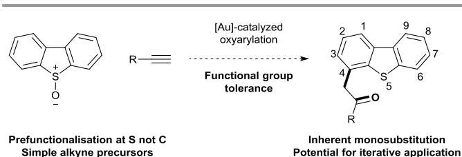
Scheme 1 Proposed regioselective functionalisation of dibenzothiophenes using the S-oxide as a traceless directing group.
