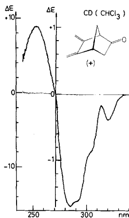
Fig. 3. CD. spectrum of (+)-7 in \text{CHCl}_3
