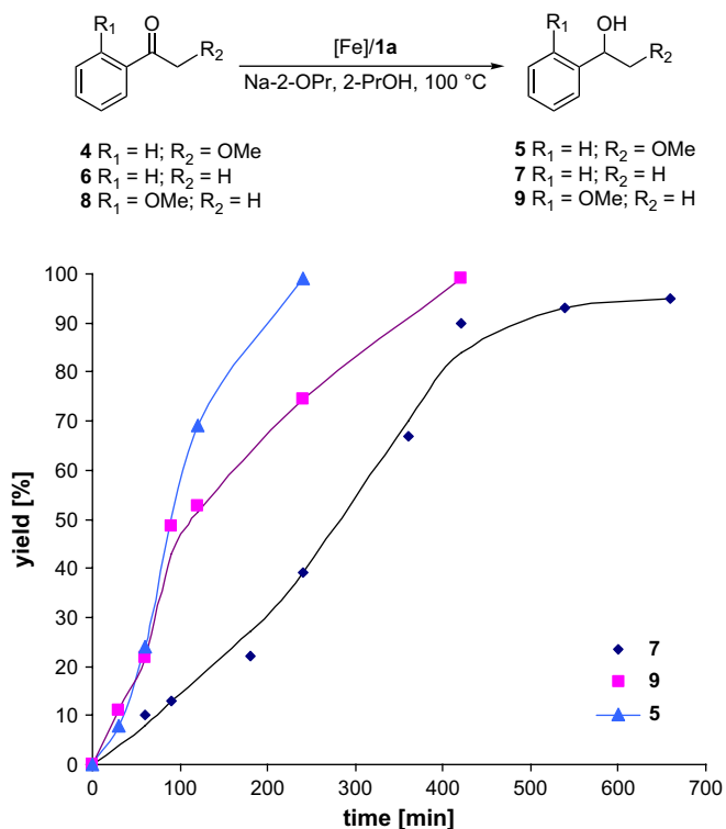
Figure 2. Comparative study between acetophenone 6 , ortho -methoxyacetophenone 8 and 2-methoxyacetophenone 4 . Reaction conditions: 0.0038 mmol in situ catalyst (0.0038 mmol \text{FeCl}_2 and 0.0038 mmol 1a in 1.0 mL 2-propanol for 16 h at 65 ^\circ\text{C} ), 0.19 mmol base in 0.5 mL 2-propanol, 0.76 mmol substrate in 0.5 mL 2-propanol, temperature: 100 ^\circ\text{C} . Yield was determined by GC analysis (7: 50 m Lipodex E, 95–150 ^\circ\text{C} , 7: 50 m Lipodex E, 90–180 ^\circ\text{C} , 9: 30 m HP Agilent Technologies 50–300 ^\circ\text{C} ) with diglyme as internal standard.
