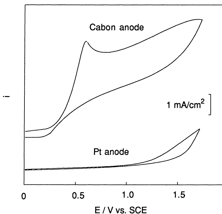
Fig. 1. Cyclic voltammograms of NaCN/MeOH at carbon and platinum anode.
