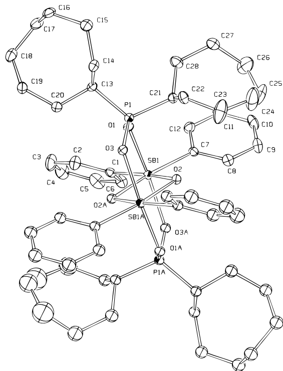
Figure 2. Molecular structure of 3 . H atoms and the solvent molecule not shown.
