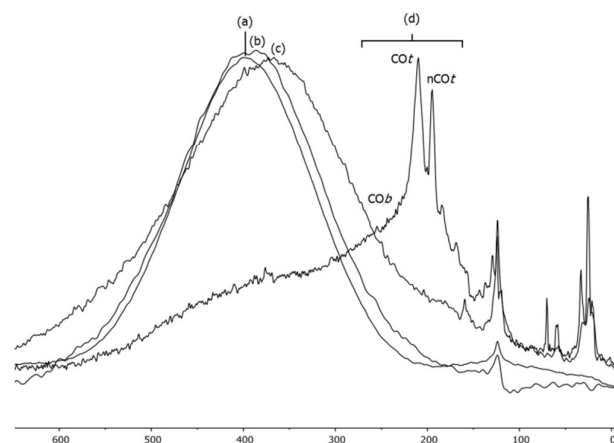
Figure 5. ^{13}\text{C} MAS NMR spectrum of (a) Pt/ICy (p-tol) NCN 0.1 (2.3 nm), (b) Pt/ICy (p-tol) NCN 0.2 (2.1 nm), (c) Pt/ICy (p-tol) NCN 0.5 (1.9 nm) and (d) Pt/CO/ICy (p-tol) NCN 0.2 (1.2 nm) after exposure to ^{13}\text{CO} (1 bar, 20 h, at r.t.)
