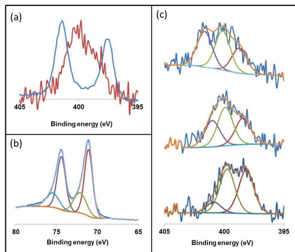
Figure 7. X-ray photoelectron spectroscopy (XPS) of (a) the N 1s signals of ICy (p-tol) NCN (blue) and Pt/ICy (p-tol) NCN 0.2 (red), (b) the Pt 4f 5/2 and 4f 7/2 signals of Pt/ICy (p-tol) NCN 0.2 and (c) the N 1s signals of Pt/ICy (p-ClC 6 H 4 ) NCN 0.2 (top), Pt/ICy (p-tol) NCN 0.2 (center) and Pt/ICy (p-anisyl) NCN 0.2 .
