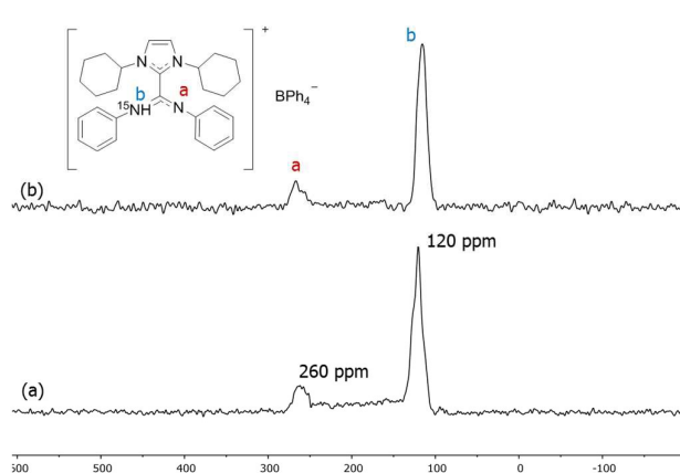
Figure 6. ^{15}\text{N} CP/Hahn-echo MAS of (a) Pt/CO/ICy (Ph) NC 15 N 0.2 and (b) [ICY (Ph) NC 15 NH] + [BPh 4 ] - .
