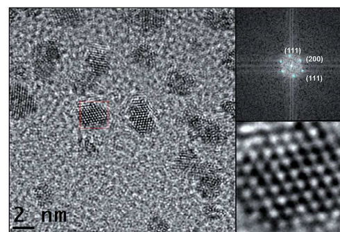
Figure 2. HRTEM image of Pt/ICy (p-tol) NCN 0.2 (left, right bottom) and Fast Fourier Transformation Analysis (right, top) with the planar reflections.
