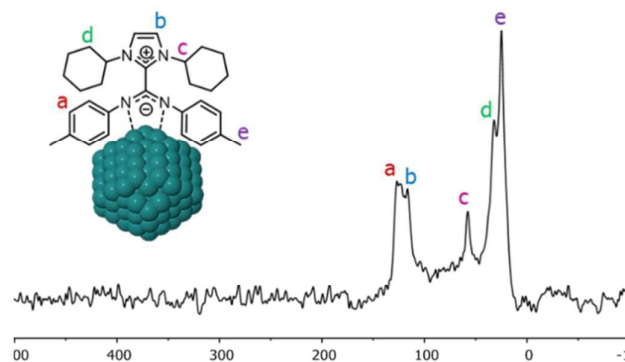
Figure 4. 13 C CP-MAS NMR spectrum of Pt/ICy (p-tol) NCN 0.5 NPs.
