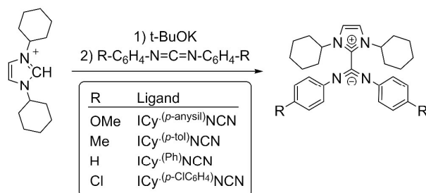
Scheme 1. Synthesis of zwitterionic imidazolium-amidinate ligands.
