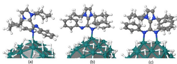
Figure 10. Coordination modes of \text{ICy}^{(\text{Ph})}\text{NCN} at the \text{Ru}_{55}\text{H}_{70} surface (a) \kappa^1\text{N} monocoordinated Z/E conformer ( E_{\text{ads}}: -25.0 kcal.mol ^{-1} ); (b) \kappa^1\text{N} monocoordinated Z/Z conformer ( E_{\text{ads}}: -33.3 kcal.mol ^{-1} ); (c) \mu_2\text{-}\kappa^1\text{N} , \kappa^1\text{N}' bicoordinated Z/Z conformer ( E_{\text{ads}}: -47.9 kcal.mol ^{-1} ).
