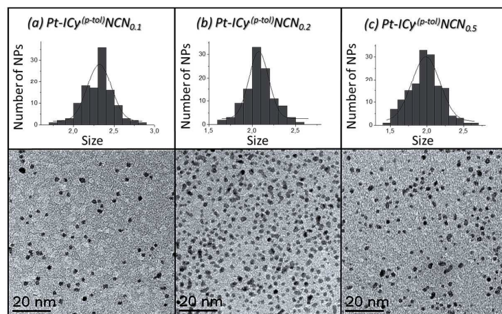
Figure 1. TEM images and size histograms of (a) Pt/ICy (p-tol) NCN 0.1 , (b) Pt/ICy (p-tol) NCN 0.2 and (c) Pt/ICy (p-tol) NCN 0.5 .
