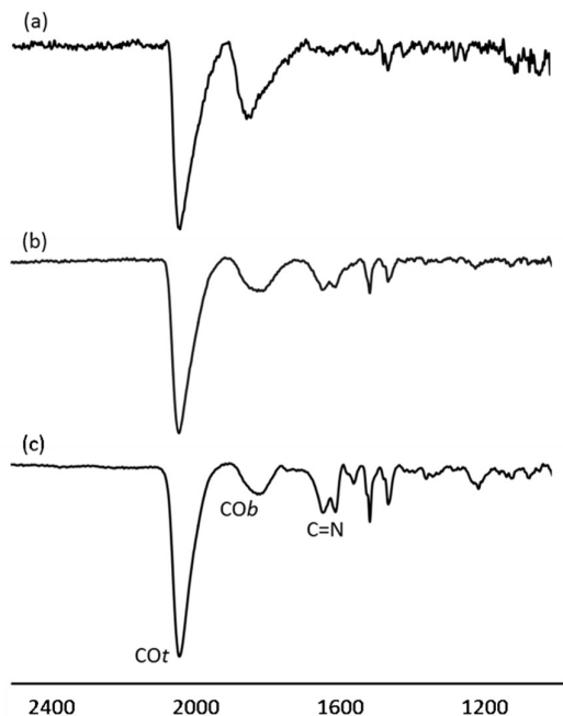
Figure 3. ATR FT-IR spectra of (a) Pt/ICy (p-tol) NCN 0.1 , (b) Pt/ICy (p-tol) NCN 0.2 and (c) Pt/ICy (p-tol) NCN 0.5 after CO adsorption.
