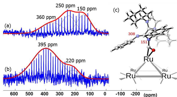
Figure 9. ^{15}\text{N} CPMG MAS NMR of \text{Ru}/\text{ICy}^{(\text{Ph})}\text{NC}^{15}\text{N}_{0.2} (a) before and (b) after exposure to ^{13}\text{CO} (1 bar, 20 h, at r.t.). (c) Calculated ^{15}\text{N} NMR displacements of \text{ICy}^{(\text{Ph})}\text{NCN} after CO insertion on a [\text{Ru}_6] cluster model.
