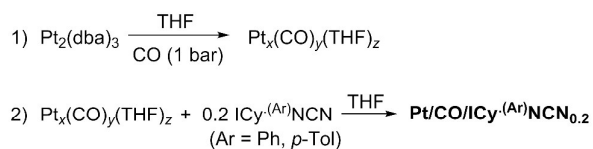
Scheme 3. Synthesis of Pt/CO/ICy (p-tol) NCN 0.2 NPs.
