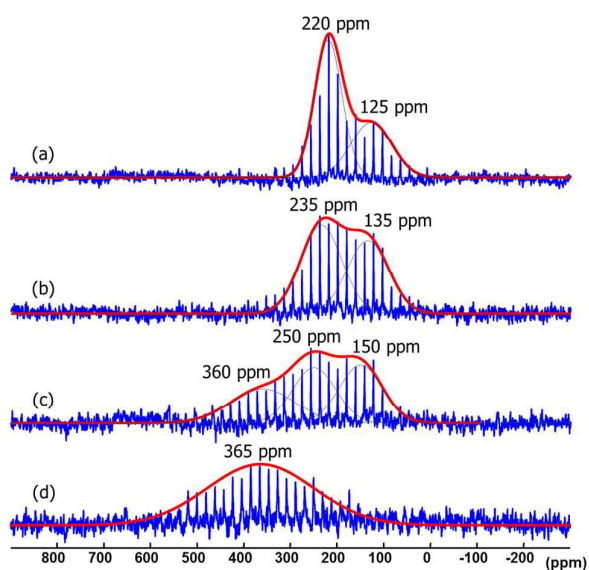
Figure 8. 15 N CPMG MAS NMR of Ru/ICy (Ph) NC 15 N stabilized with (a) 1 equiv., (b) 0.5 equiv., (c) 0.2 equiv. and (d) 0.1 equiv.
