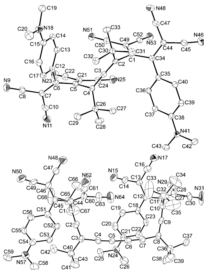
Figure 5. ORTEP plot of ( \pm )- 6 (top, T=170 K) and ( M,M )- 11 (bottom, T=220 K) with vibrational ellipsoids shown at the 30% probability level. Arbitrary numbering. Selected dihedral angles [ ^\circ ]: ( \pm )- 6 : C3–C4–C5–C21 71.9(3), C3–C4–C5–C6 -106.0(2) , C21–C5–C6–C7 58.4(3), C12–C6–C7–C8 8.7(4), C49–C1–C2–C3 65.8(3), C34–C1–C2–C3 -113.2(2) , C49–C1–C34–C44 65.4(3), C35–C34–C44–C45 3.6(4); ( M,M )- 11 : C2–C1–C44–C60 -77.6(12) , C2–C1–C44–C45 98.4(10), C60–C44–C45–C46 -70.2(14) , C51–C45–C46–C49 -0.6(16) , C9–C10–C11–C27 101.8(12), C9–C10–C11–C12 -74.1(11) , C27–C11–C12–C13 73.3(13), C18–C12–C13–C14 7.4(14) (see Supporting Information).
