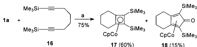
Scheme 2. Attempted cycloaddition of 1a to 1,8-bis(trimethylsilyl)-1,7-octadiyne 16 . Reagents and conditions: a) [\text{CpCo}(\text{CO})_2] (1.5 equiv), h\nu , toluene, 40 °C, 30 h.
