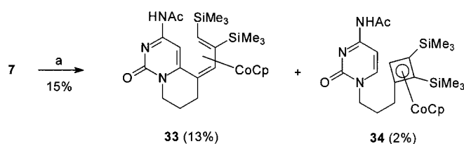
Scheme 5. Cycloaddition of 7 with BTMSA. Reagents and conditions: a) [CpCo(CO) 2 ] (2 equiv), BTMSA (6 equiv), hν , THF, RT, 20 h.
