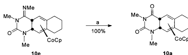
Scheme 3. Hydrolysis of 10e . Reagents and conditions: a) \text{SiO}_2 , MeOH or \text{Al}_2\text{O}_3 , \text{H}_2\text{O} , RT.
