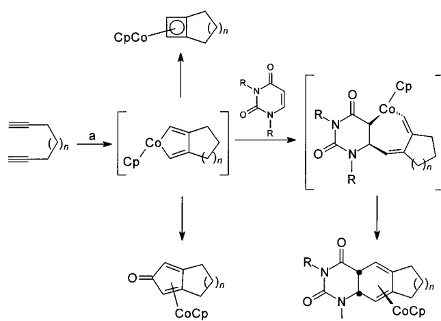
Scheme 7. Proposed mechanism for intermolecular cycloadditions.
