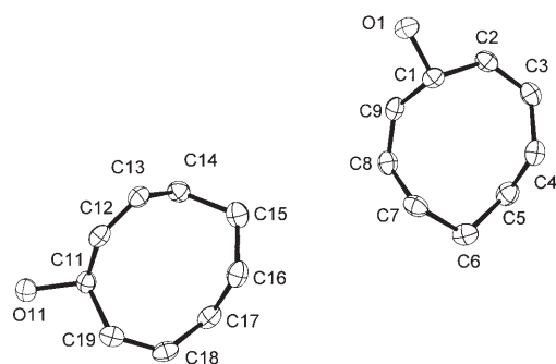
Figure 4. Molecular crystal structure of cyclononadienol 20 in the solid state (two independent molecules in the unit cell). Anisotropic displacement parameters are drawn at the 50% probability level.
