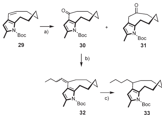
Scheme 7. Elaboration of the core region: a) i) \text{BH}_3\cdot\text{THF} , THF, -10^\circ\text{C} ; ii) \text{Me}_3\text{N}/\text{THF} , aq. NaOH (3 M), \text{H}_2\text{O}_2 , 0^\circ\text{C} ; iii) Dess-Martin periodinane, 65 % (2–5:1 ratio); b) \text{Ph}_3\text{P}=\text{CHCH}_2\text{CH}_2\text{CH}_3 , toluene, reflux, 75 %; c) \text{H}_2 (1 atm), [(\text{cod})(\text{pyridine})\text{Ir}(\text{PCy}_3)]\text{PF}_6 (10 mol %), \text{CH}_2\text{Cl}_2 , 90 %.
