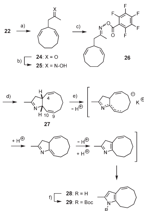
Scheme 6. a) Aq. DMSO, 180 °C, 99%; b) H 2 NOH·HCl, NaOAc, aq. EtOH, 100 °C, 97%; c) pentafluorobenzoylchloride, Et 3 N, Et 2 O, –78 °C → RT, 97%; d) Pd(OAc) 2 (12 mol %), ( o -tolyl) 3 P (12 mol %), Et 3 N, DMF, 110 °C, 54%; e) KH, 1,3-diaminopropane, 65%; f) Boc 2 O, DMAP (10 mol %), MeCN, 50 °C, 69%.
