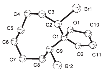
Figure 2. Molecular crystal structure of dibromide 15 in the solid state. Anisotropic displacement parameters are drawn at the 50% probability level.
