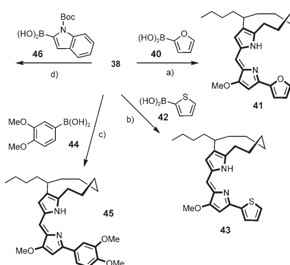
Scheme 9. Preparation of analogues: a) boronic acid 40 , catalytic [\text{Pd}(\text{PPh}_3)_4] , LiCl, aq. \text{Na}_2\text{CO}_3 , DME, 80 °C, 81 %; b) boronic acid 42 , catalytic [\text{Pd}(\text{PPh}_3)_4] , LiCl, aq. \text{Na}_2\text{CO}_3 , DME, 80 °C, 81 %; c) boronic acid 44 , catalytic [\text{Pd}(\text{PPh}_3)_4] , LiCl, aq. \text{Na}_2\text{CO}_3 , DME, 80 °C, 44 %; d) boronic acid 46 , catalytic [\text{Pd}(\text{PPh}_3)_4] , LiCl, aq. \text{Na}_2\text{CO}_3 , DME, 80 °C, 72 %.
