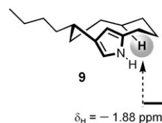
Scheme 1. High-field shift of an aliphatic proton as a characteristic signature of the 1 H NMR spectra of compounds with a rigid meta -pyrrolophane structure.
