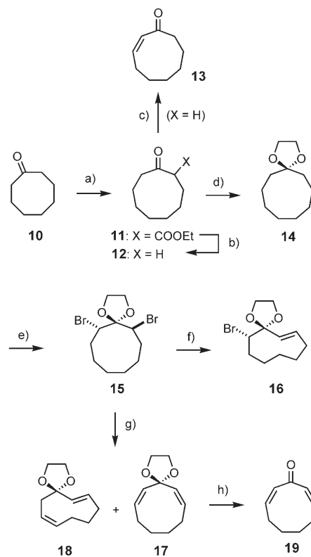
Scheme 4. Large-scale adaptable synthesis of cyclononadienone 19 : a) ethyl diazoacetate, \text{Et}_3\text{O}^+\text{BF}_4^- , \text{CH}_2\text{Cl}_2 , 0^\circ\text{C} , 64%; b) aq. DMSO, 150^\circ\text{C} , 83–86%; c) IBX, toluene/DMSO, 80^\circ\text{C} , 76%; d) ethyleneglycol, catalytic pyridinium p -toluenesulfonate (PPTS), benzene, reflux, 75–92%; e) \text{Br}_2 , \text{Et}_2\text{O} , 0^\circ\text{C} \rightarrow \text{RT} , 76–84%; f) KOH, toluene, reflux, 64%; g) t BuOK, DMSO, 85^\circ\text{C} , 96% (purity: \geq 80\% 17 + \approx 11\% 18 , rest: other isomers); h) catalytic PPTS, aq. acetone, pyridine, 55^\circ\text{C} , 45–56% ( > 99\% pure).
