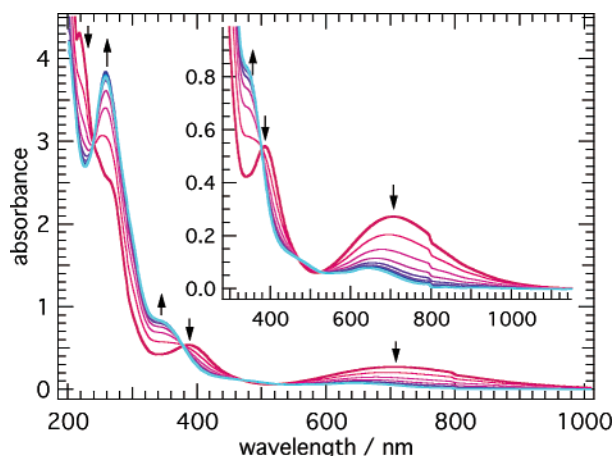
Figure 7. UV-vis-NIR spectroelectrochemistry for controlled-potential oxidation of 3 at +0.90 V (vs \text{Fc}^+/\text{Fc} ) in acetonitrile-0.2 M [\text{Bu}_4\text{N}][\text{PF}_6] at 298 K.
