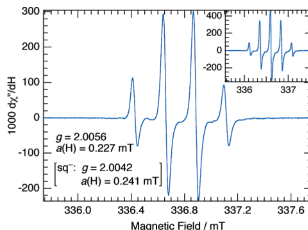
Figure 9. X-band EPR spectrum of \text{Fc-sq}^- obtained during in situ electrolysis of 3 at -1.0 V (vs \text{Fc}^+/\text{Fc} ) in acetonitrile-0.1 M [\text{Bu}_4\text{N}][\text{PF}_6] at 298 K. Inset: X-band EPR spectrum of the semiquinone ( \text{sq}^- ) anion obtained from 1,4-benzoquinone under identical conditions.
