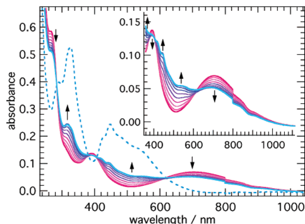
Figure 8. UV-vis-NIR spectroelectrochemistry for reduction of 3 at -1.0 V (vs \text{Fc}^+/\text{Fc} ) in acetonitrile-0.2 M [\text{Bu}_4\text{N}][\text{PF}_6] at 298 K. The changes are ( \sim 85\% ) reversed by electrolysis at -0.15 V. The spectrum of the reduction product (dashed trace) was obtained by normalizing the first ( 3 ) spectrum and the final (reduction product + 3 ) spectrum at 705 nm, subtracting the normalized first spectrum from the normalized final spectrum, and then scaling the absorbances so that they match those in all spectra at the isosbestic points.
