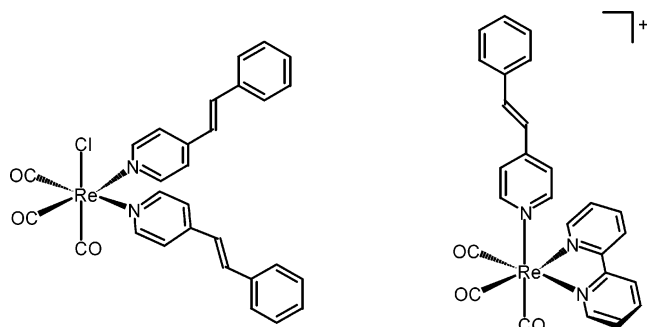
Figure 1. Schematic structures of \text{fac}[\text{Re}(\text{Cl})(\text{CO})_3(\text{stpy})_2] (left) and \text{fac}[\text{Re}(\text{stpy})(\text{CO})_3(\text{bpy})]^+ (right).
