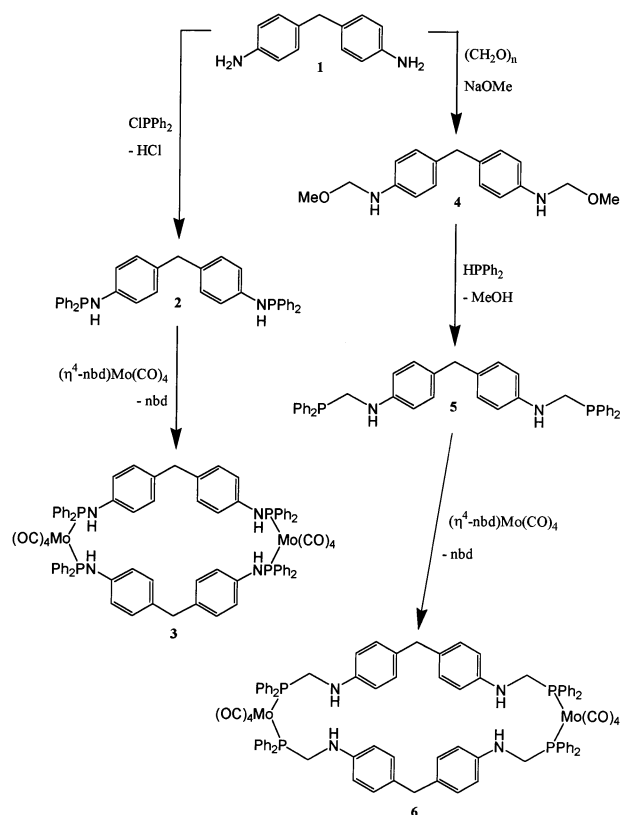
Scheme 1. Synthesis of the aminophosphines 2 and 5 and the dimolybdacyclophanes 3 and 6 .
