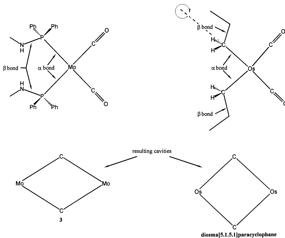
Fig. 3. Schematic view onto the transition metal fragments of compound 3 and the diosma[5.1.5.1]paracyclophane along the axial CO ligands.
