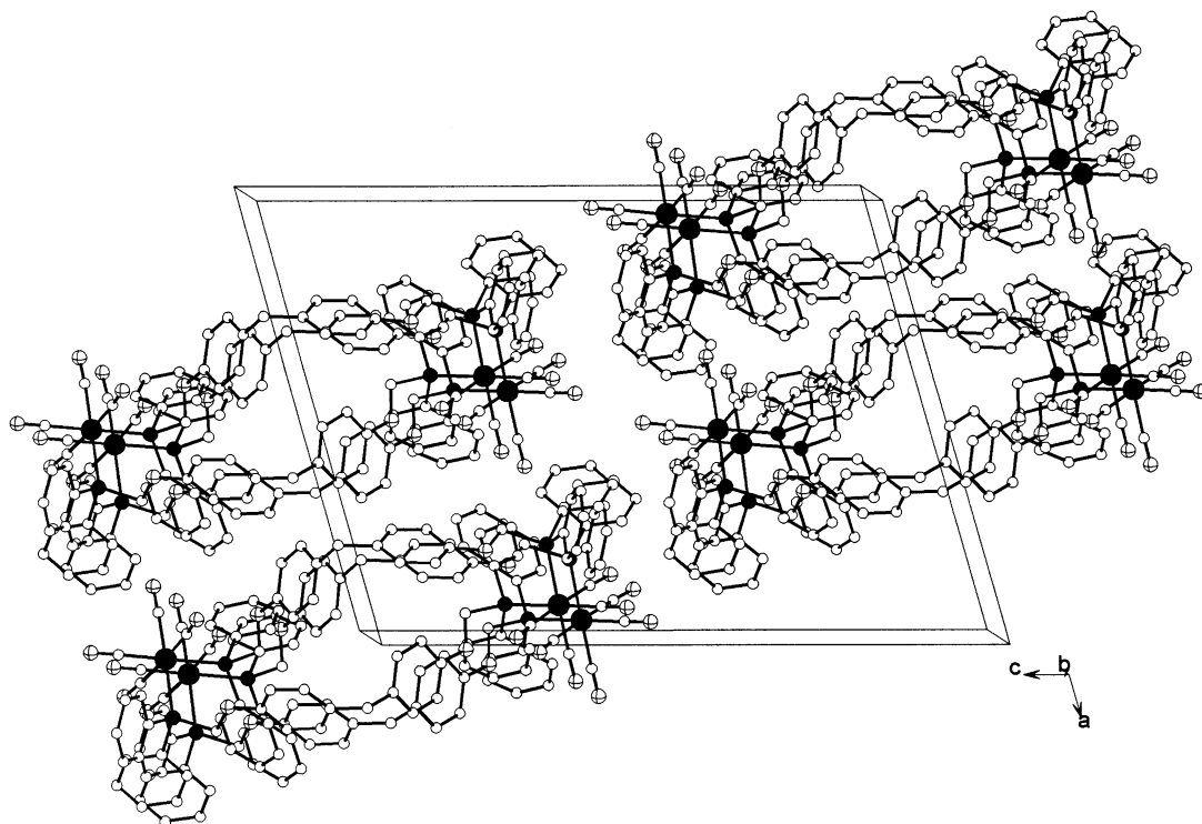
Fig. 5. Four channels of molecules of 6 viewed along the b axis. Solvent molecules are omitted for clarity, unit cell is shown.
