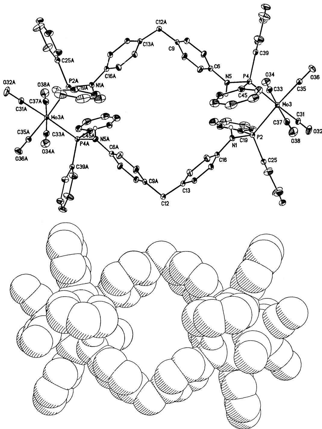
Fig. 1. Top: ORTEP plot of the molecular structure of compound 3 . Thermal ellipsoids are drawn at 20% probability level, except for H atoms. Phenyl rings are numbered cyclically. Bottom: space-filling representation of 3 . Solvent molecules are omitted for clarity.
