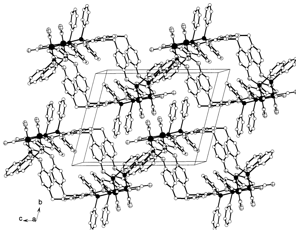
Fig. 2. Four channels of molecules in the crystal structure of 3 viewed along the a axis. Solvent molecules are omitted for clarity, unit cell is shown.
