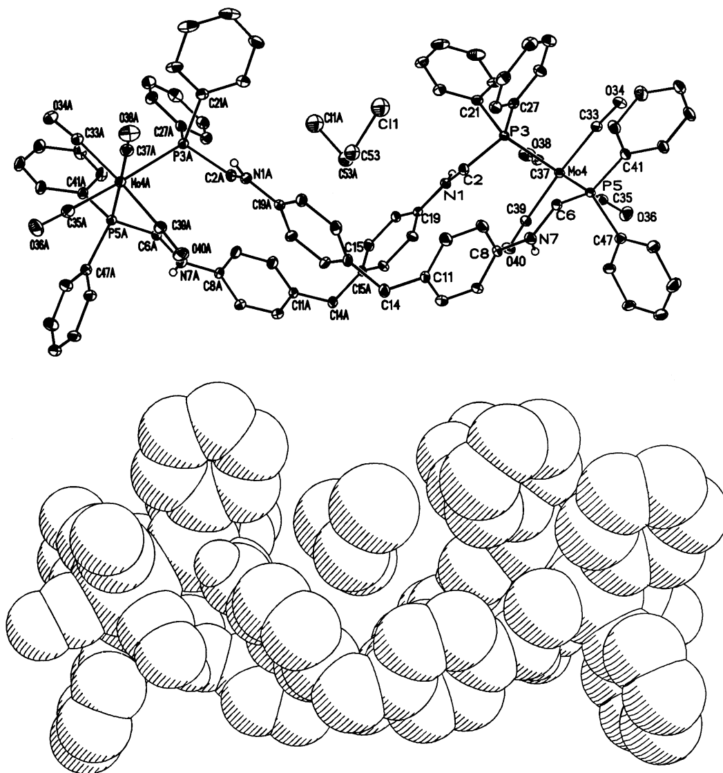
Fig. 4. Top: ORTEP plot of the molecular structure of compound 6 . Thermal ellipsoids are drawn at 20% probability level, except for H atoms. Phenyl rings are numbered cyclically. Bottom: space-filling representation of 6 . Solvent molecules that are located outside the cavity are omitted for clarity.
